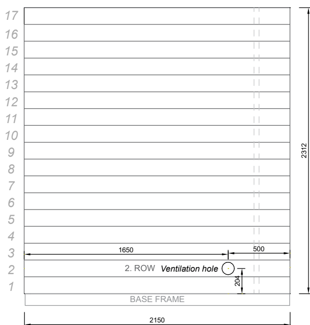
Scheme 6.1
