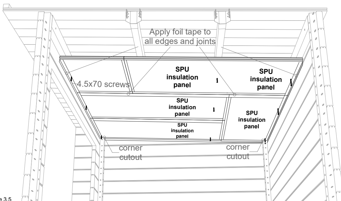
Scheme 3.5
