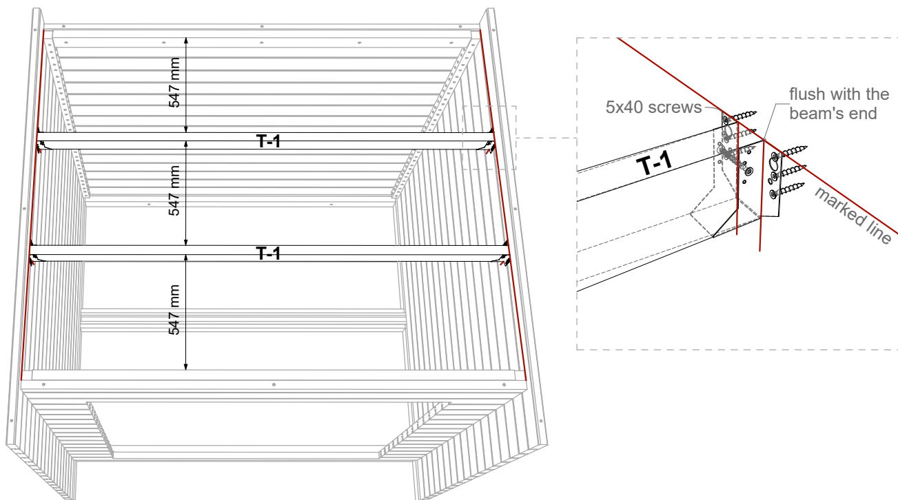
Scheme 3.3
