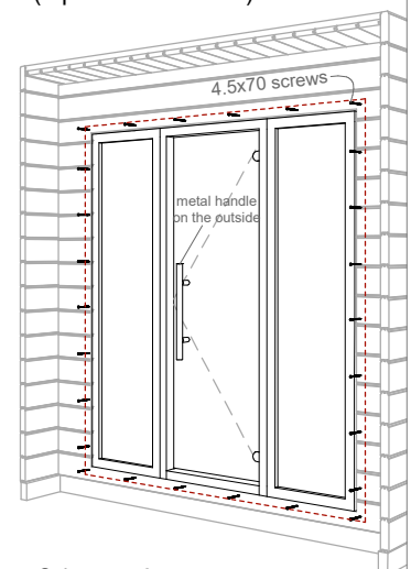
Scheme 5.3
