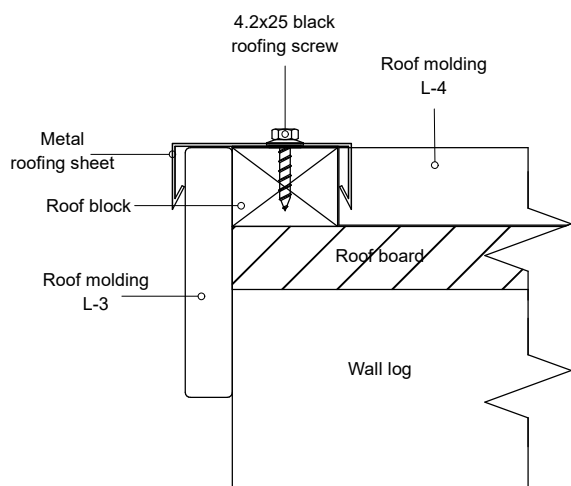
Scheme 10.5
