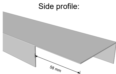
Scheme 10.2
