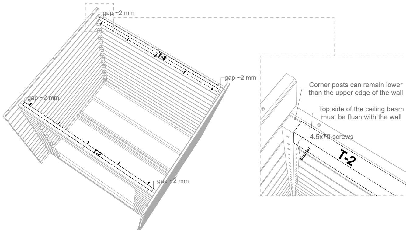
Scheme 3.1
