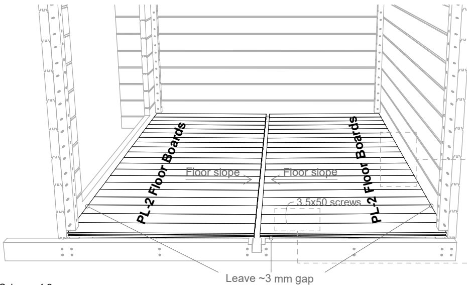
Scheme 4.2
