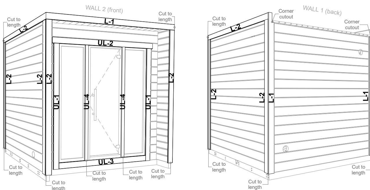
Scheme 7.3
