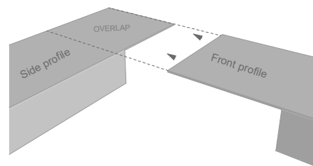
Scheme 10.4
