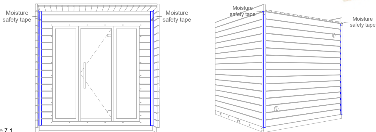
Scheme 7.1
